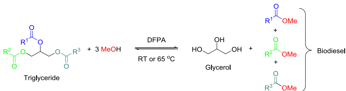
Scheme 1. Synthesis of FAME from soybean oil using DFPA
