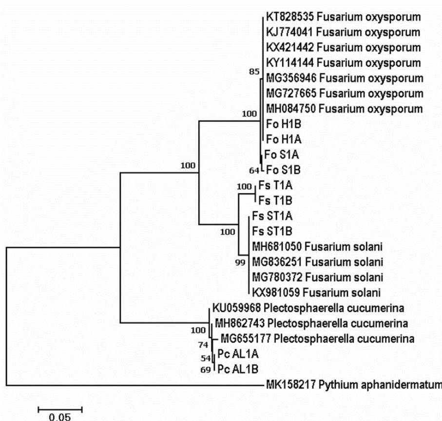
Figure 4 | Evolutionary phylogenetic relationship of the fungal isolates based on ITS ribosomal DNA sequences constructed using the neighbor-joining method. Bootstrap tests were performed with 1,000 replications; and the percentage value greater than 50 is considered a strong support for a branch. Pythium aphanidermatum (MK158217) obtained from GenBank was treated as the outgroup.
