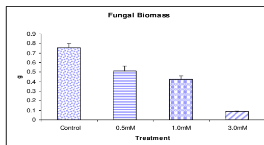
Fig.2: Fungal Biomass
