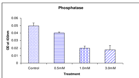
Fig.3: Phosphatase
