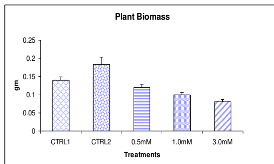
Fig.4: Plant Biomass
