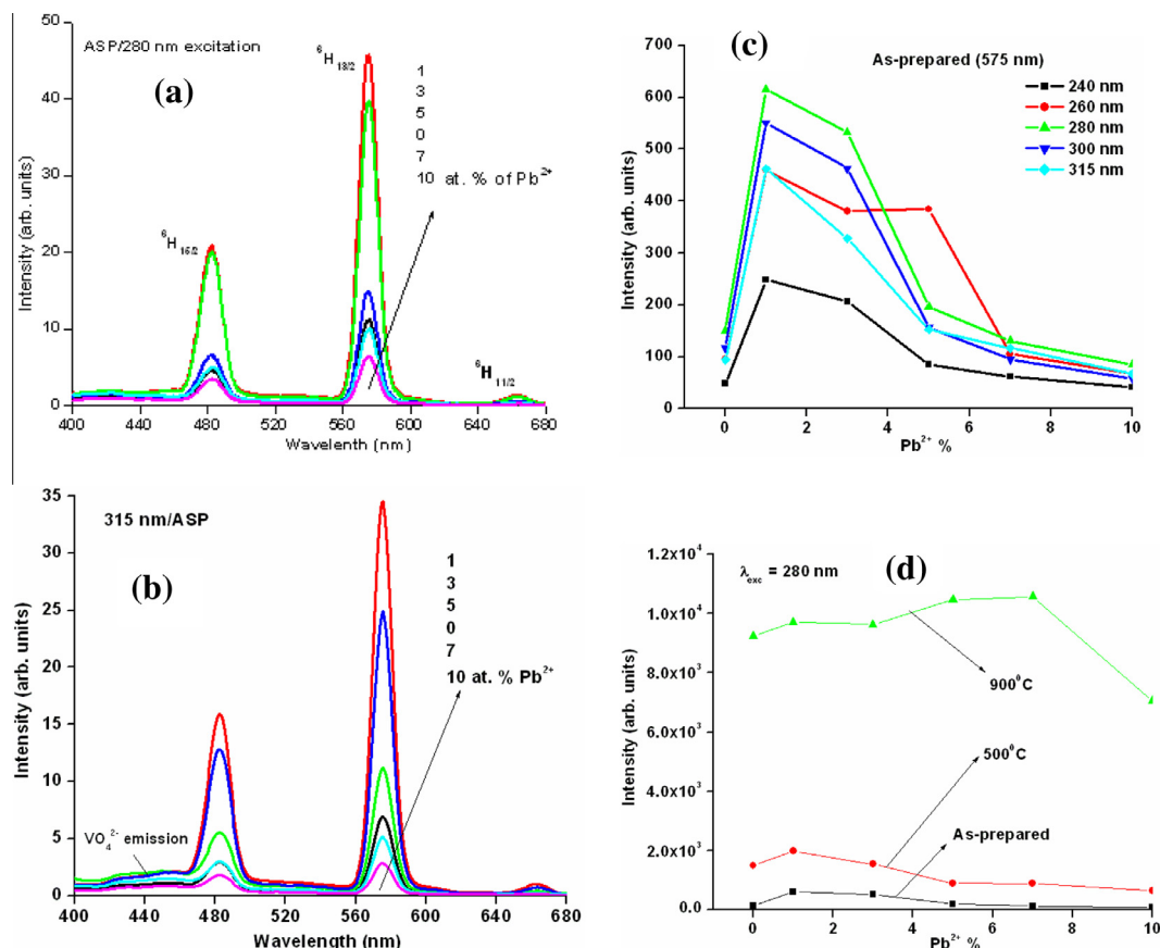
Fig. 6. Emission spectra of as-prepared Pb^{2+} co-doped YVO_4:5Dy^{3+} nanoparticles ( Pb^{2+} = 0, 1, 3, 5, 7 and 10 at.%) under excitation wavelength at (a) 280 nm and (b) 315 nm. (c) Plot of integrated area vs concentration of Pb^{2+} for as-prepared at different excitation wavelengths. (d) Plot of integrated area vs concentration of Pb^{2+} for as-prepared, 500 and 900 °C annealed samples under excitation 280 nm.
