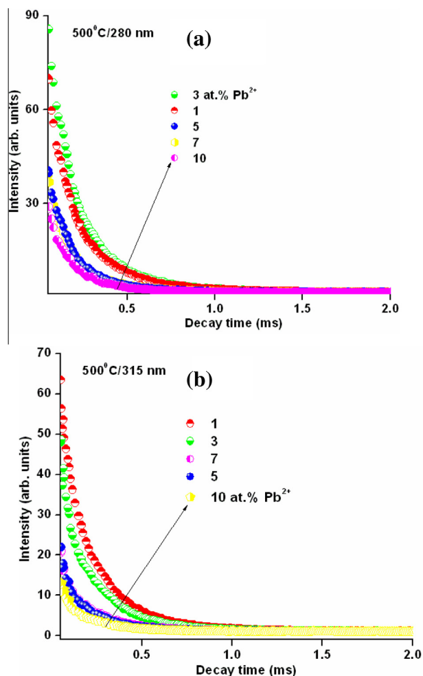
Fig. 11. Luminescence decay spectra of 500 °C annealed \text{Pb}^{2+} co-doped \text{YVO}_4:5\text{Dy}^{3+} nanoparticles at 280 and 315 nm excitations.
