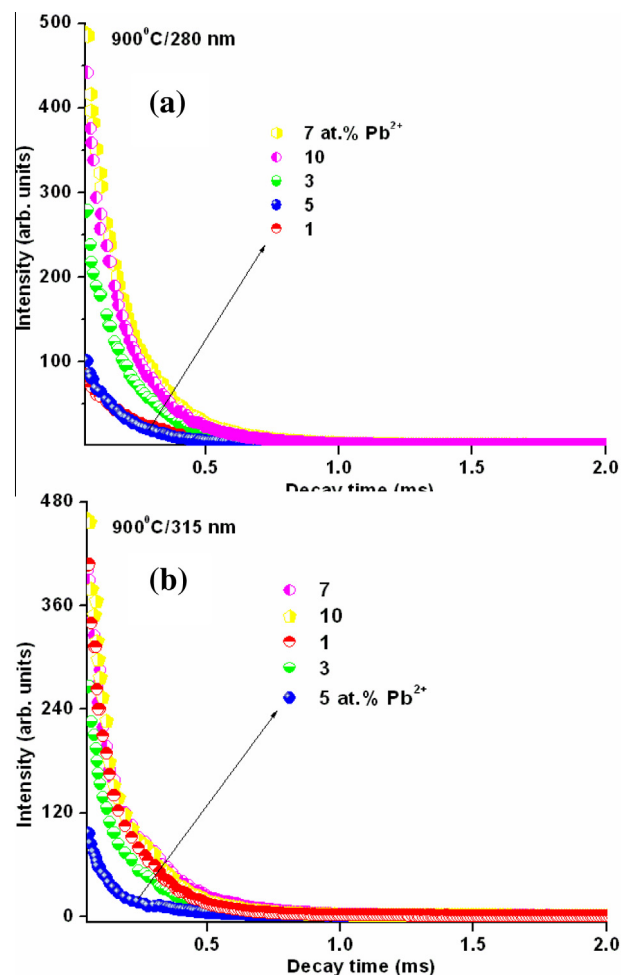
Fig. 12. Luminescence decay spectra of 900 °C annealed \text{Pb}^{2+} co-doped \text{YVO}_4:5\text{Dy}^{3+} nanoparticles at 280 and 315 nm excitations.
