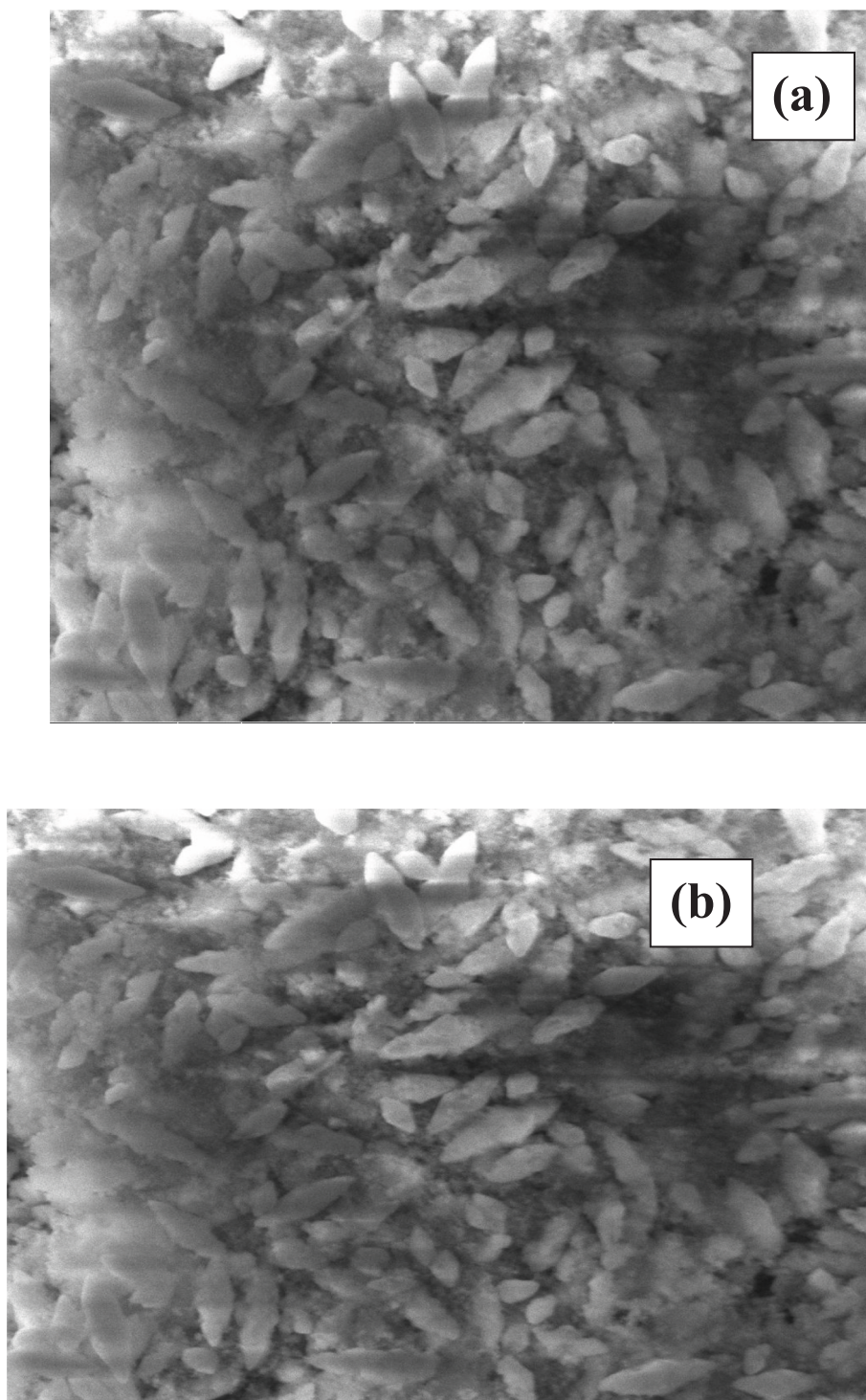
Fig. 3. SEM image of 20 at.% (a) Sm 3+ and (b) Dy 3+ -doped BaMoO 4 .
