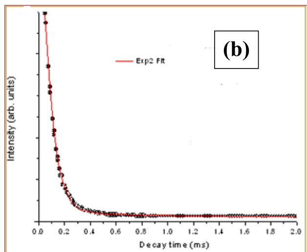
Fig. 9. Bi-exponential fitting to luminescence decay data of (a) 7at. % doped BaMoO 4 :Sm 3+ and (b) 7at. % doped BaMoO 4 :Dy 3+ nanoparticles.
