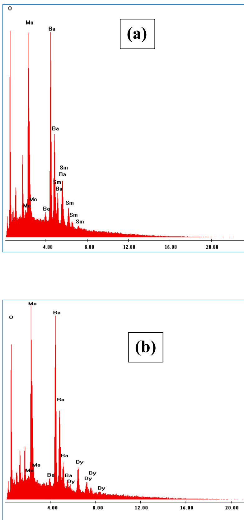
Fig. 2. EDX pattern of 20 at.% (a) Sm 3+ - and (b) Dy 3+ -doped BaMoO 4 .
