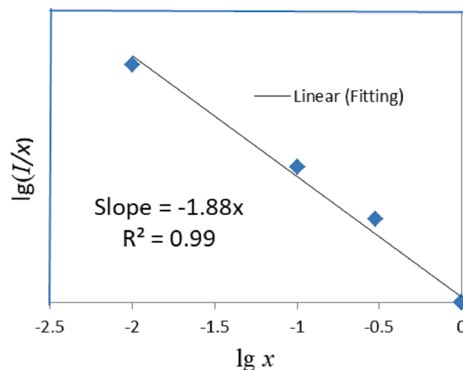
Fig. 11. The dependence of \lg(I/x) on \lg x according to Eq. (8).
