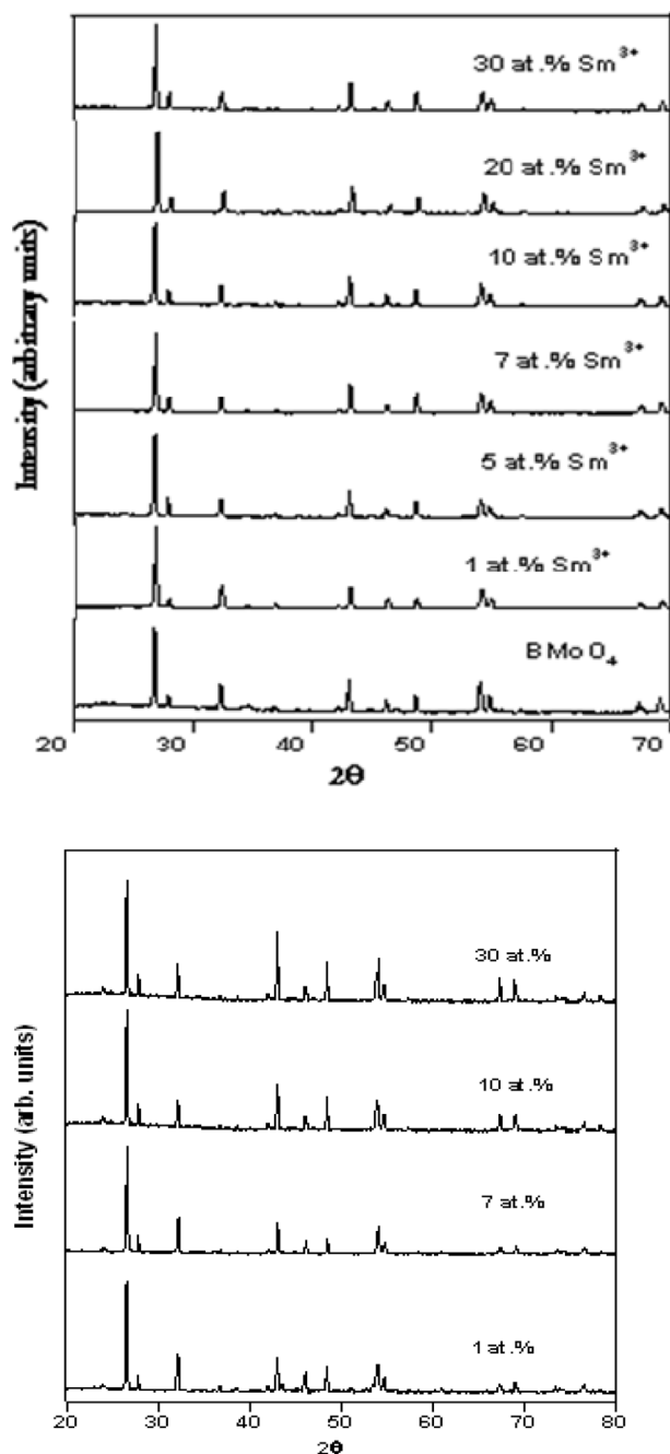
Fig. 1. XRD pattern of (a) \text{Sm}^{3+} -doped \text{BaMoO}_4 and (b) \text{Dy}^{3+} -doped \text{BaMoO}_4 ( \text{Sm}^{3+}/\text{Dy}^{3+} = 1, 3, 5, 7, 10, 20 and 30 at.%) nanoparticles.
