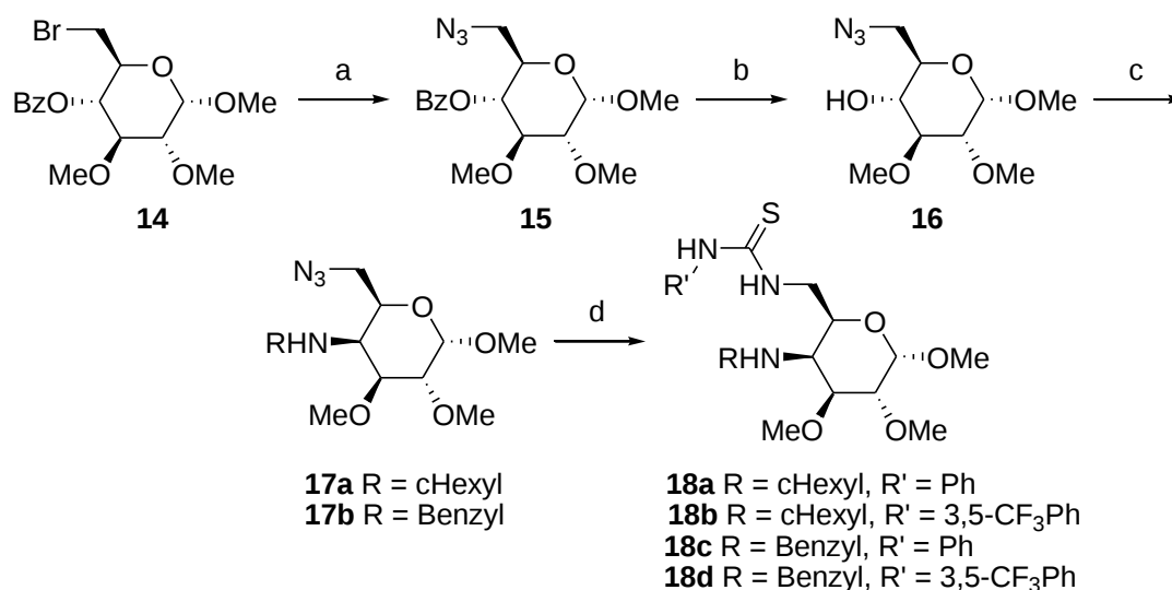
Scheme 15 | Synthesis of the catalysts; (a) \text{NaN}_3 , DMF, 70^\circ\text{C} , 6 h, 94%; (b) NaOMe, MeOH, rt, 1 h, 80%; (c) (i) \text{Tf}_2\text{O} , pyridine, \text{CH}_2\text{Cl}_2 , 0^\circ\text{C} , 2 h, (ii) amine, DMF, 45^\circ\text{C} , 10 h, 50-70%; (d) (i) propanedithiol, MeOH, rt, 48 h ( 18a and 18b ), or \text{PPh}_3 , \text{H}_2\text{O} , THF, 80^\circ\text{C} , ( 18c and 18d ), (ii) isothiocyanate, MeOH, rt, 4 h, 30-50%.
