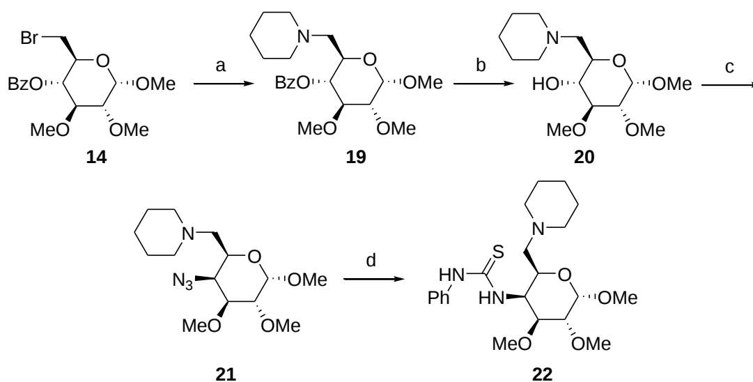
Scheme 16 | Synthesis of organocatalysts; (a) piperidine, DMF, 70^\circ\text{C} , 50 h, 90%; (b) NaOMe, MeOH, reflux, 2 h, 85%; (c) \text{Tf}_2\text{O} , pyridine, DCM, 0^\circ\text{C} , 2 h, (ii) \text{NaN}_3 , DMF, 45^\circ\text{C} , 72 h, 40%; (d) (i) propanedithiol, MeOH, rt, 48 h, (ii) phenyl isothiocyanate, MeOH, rt, 8 h, 69%.
